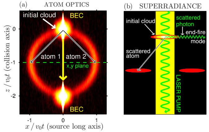
FIG. 8. (Color online) A schematic comparison of the scattering geometry in (a) atom collisions and (b) superradiance in the rest frame of the upper condensate. The color background shows the long-time atom distribution on the x - z plane. In (a), it comes from the stochastic Bogoliubov simulation for the N = 10^5 case. We use the k -space distribution at the end of the collision, scaled out to the far field via x = (\hbar k/m)t . The x - y plane analyzed in the text is shown as a dashed green line. In both panels, arrows show flight paths.
