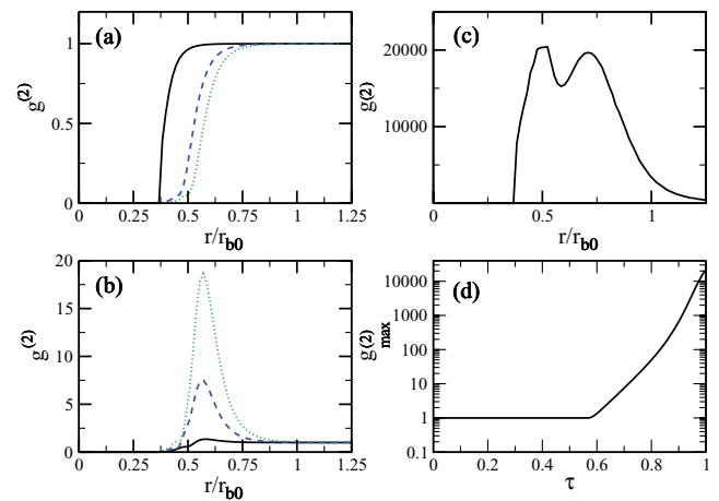
FIG. 2. (Color online) Spatial atomic correlations during an echo sequence with \rho_0 V_{b0} = 5.4 . (a) Pair correlation function g^{(2)}(r) during the excitation phase at \tau = 0.05 (solid black line), \tau = 0.37 (blue dashed line) and \tau = 0.49 (green dotted line). Below the cutoff length r_{\text{cut}} , g^{(2)} is set to zero [22]. (b) The same during the deexcitation phase at \tau = 0.6 (solid black line), \tau = 0.7 (blue dashed line) and \tau = 0.75 (green dotted line). (c) Final shape of the pair correlation function after the pulse ( \tau = 1 ). (d) Spatial maximum of pair correlations. The location of the time samples in panels (a)–(c) relative to the pulse can be seen clearly in Fig. 1.
