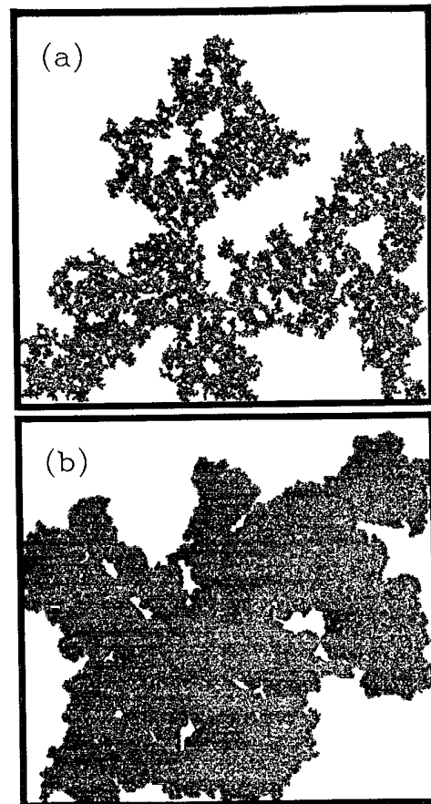
FIG. 2. Percolating patterns for sample A with L=300 and (a) \theta=179^\circ , and (b) \theta=58^\circ . The invading fluid is black, disks and invaded fluid are white.
