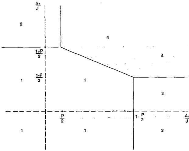
FIG. 1. T=0 phase diagram in the \Delta_0/J - \Delta_1/J plane.
