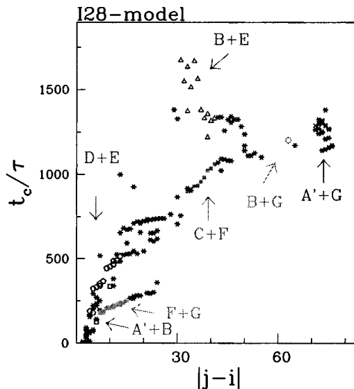
FIG. 5. Same as in Fig. 4 but for I28-model.
