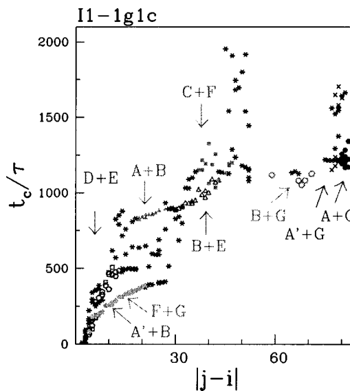
FIG. 6. Same as in Fig. 4 but for I1-1g1c.
