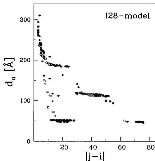
FIG. 13. The scenario of stretching for I28-model at \tilde{T}=0.3 .
