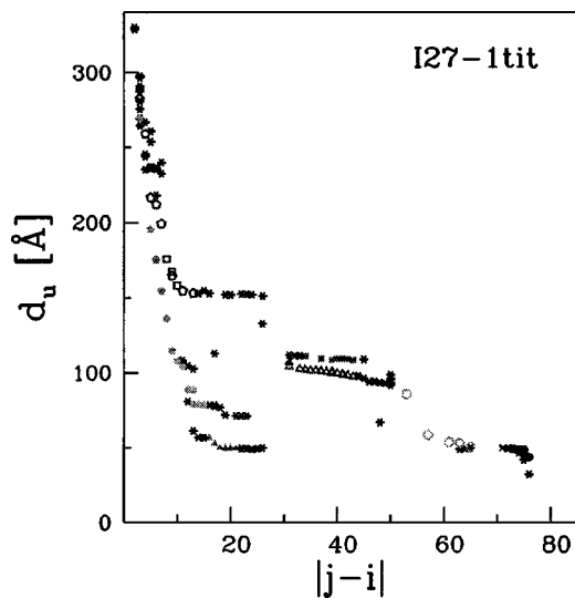
FIG. 12. Same as in Fig. 9 but for \tilde{T}=0.3 . The data points are averaged over 20 trajectories.
