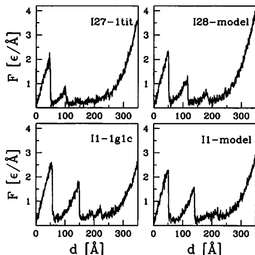
FIG. 8. Same as in Fig. 4 but for \tilde{T}=0.3 which should correspond to the room temperature situation. The pulling force is averaged over 100\tau , i.e., over the distance of 0.5 \text{ \AA} , to reduce the random noise.
