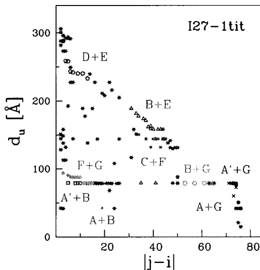
FIG. 9. The scenario of mechanical unfolding at \tilde{T}=0 for I27-1tit. The data points show the last distance at which particular contacts are considered to be still holding. The letter symbols are as in Fig. 4.
