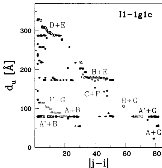
FIG. 11. Same as in Fig. 9 but for I1-1g1c.
