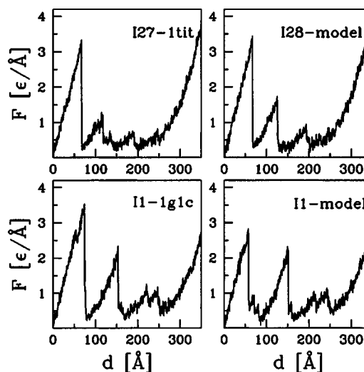
FIG. 19. An analog of Fig. 6 at \tilde{T} = 0.3 for a generalized model in which the hydrophobic-hydrophobic contacts are made stronger by a factor of 2.
