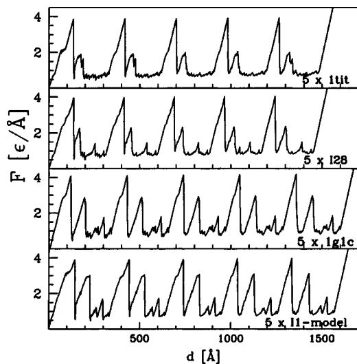
FIG. 16. Stretching of five domains of titin, linked in a tandem arrangement as listed in each panel, at \tilde{T}=0 .
