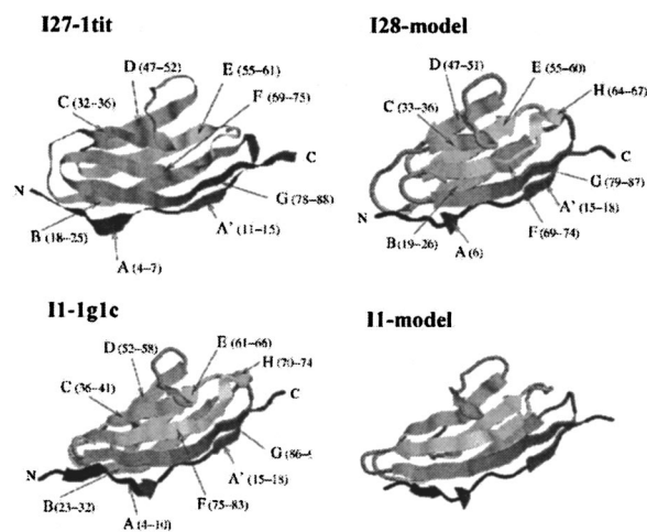
FIG. 1. The structures of the domains of titin studied in this paper. The labeling of the \beta strands (symbols A through G) is indicated, together with the allocation of the amino acids to the structures. The fragments corresponding to the \alpha helix are denoted by H .
