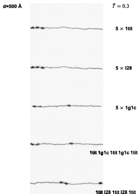
FIG. 18. Snapshots of the five-domain arrangements when stretched by 500 Å. The top-to-bottom ordering of the snapshots corresponds to the one adopted in Fig. 11.
