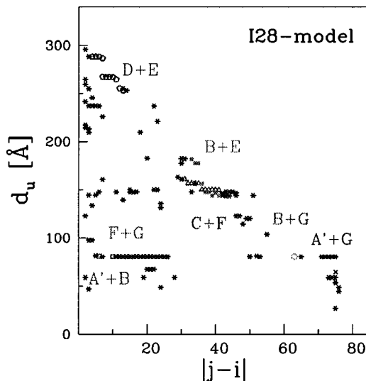
FIG. 10. Same as in Fig. 9 but for I28-model.
