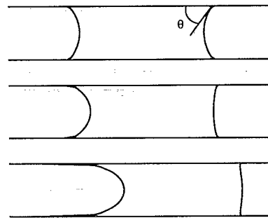
FIG. 18. A blob within two partially wetting walls with three different velocities V = 0.489 \times 10^{-3} , 4.58 \times 10^{-3} , and 9.5 \times 10^{-3} increasing from top to bottom (CA units).
