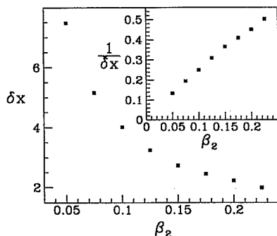
FIG. 7. Interface thickness \delta x in lattice units, versus the control parameter \beta_2 . The inset shows that the inverse thickness depends on \beta_2 in a linear fashion.
