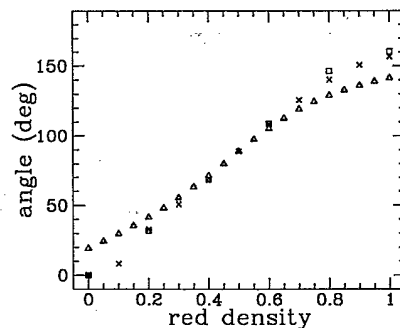
FIG. 15. Plot of the contact angle versus the relative color content of the wall. Triangles, crosses, and squares show the situation after 6000, 18 000, and 60 000 time steps, respectively.
