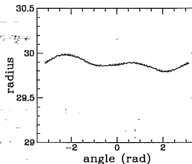
FIG. 5. Radius of the circular blob of Fig. 4 versus the polar angle ( -\pi, \pi ). The fluctuations ( \sim 0.1 ) in the effective radius are small compared to the average radius (30).
