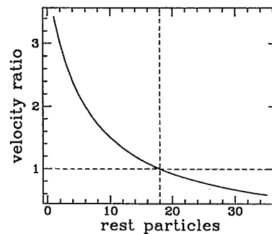
FIG. 1. Plot of the velocity ratio (velocity of moving particles v_{flow} divided by the shear wave velocity v_{sw} ) versus the number of rest particles. The reduced density in each cell is 1/3 . The dashed lines show that Galilean invariance is restored, v_{flow}/v_{sw} = 1 , for 18 rest particles as expected.
