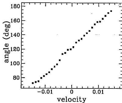
FIG. 20. Same as Fig. 19 but for the partially nonwetting case: the static contact angle is 135^\circ .
