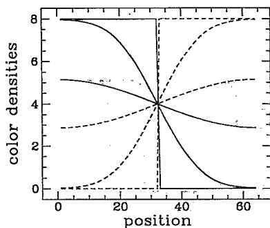
FIG. 3. The situation corresponding to complete miscibility: \beta_1 = 0 and \beta_2 = 0 . An initially sharp interface ( t = 0 ) vanishes due to "molecular" diffusion. The red and blue state densities are plotted versus position (lattice units) for time steps 1000 and 10 000.
