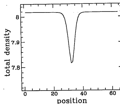
FIG. 8. Plot of the total state density (red+blue) on a line crossing an interface. \beta_1 = 0.0015 and \beta_2 = 0.15 . The interface region shows a decrease of the total density, accounting for the surface tension.
