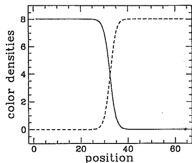
FIG. 6. Red (solid line) and blue (dashed line) state densities are plotted on a line crossing an interface. The values of our control parameters are \beta_1 = 0.0015 and \beta_2 = 0.15 .
