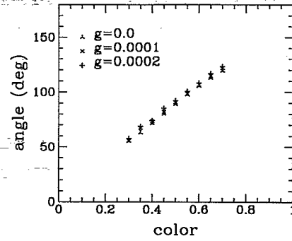
FIG. 17. Plots of the contact angle versus the relative color content for various gravity fields.
