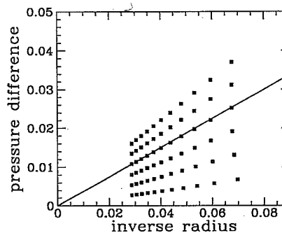
FIG. 9. For several bubble radii and six values of \beta_1 ( \beta_1 = 0.0005, 0.001, \dots, 0.003 and \beta_2 = 100\beta_1 ), we have measured the pressure difference between the inside and the outside of the bubble. For each value of \beta_1 , a straight line through the points crosses the axis close to the origin, as shown for \beta_1 = 0.002 . The slope of this line is the surface tension (CA units).
