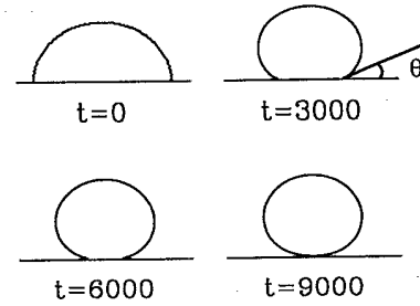
FIG. 14. Dewetting of a drop placed on a wall surface of opposite color, shown at various times of the evolution.
