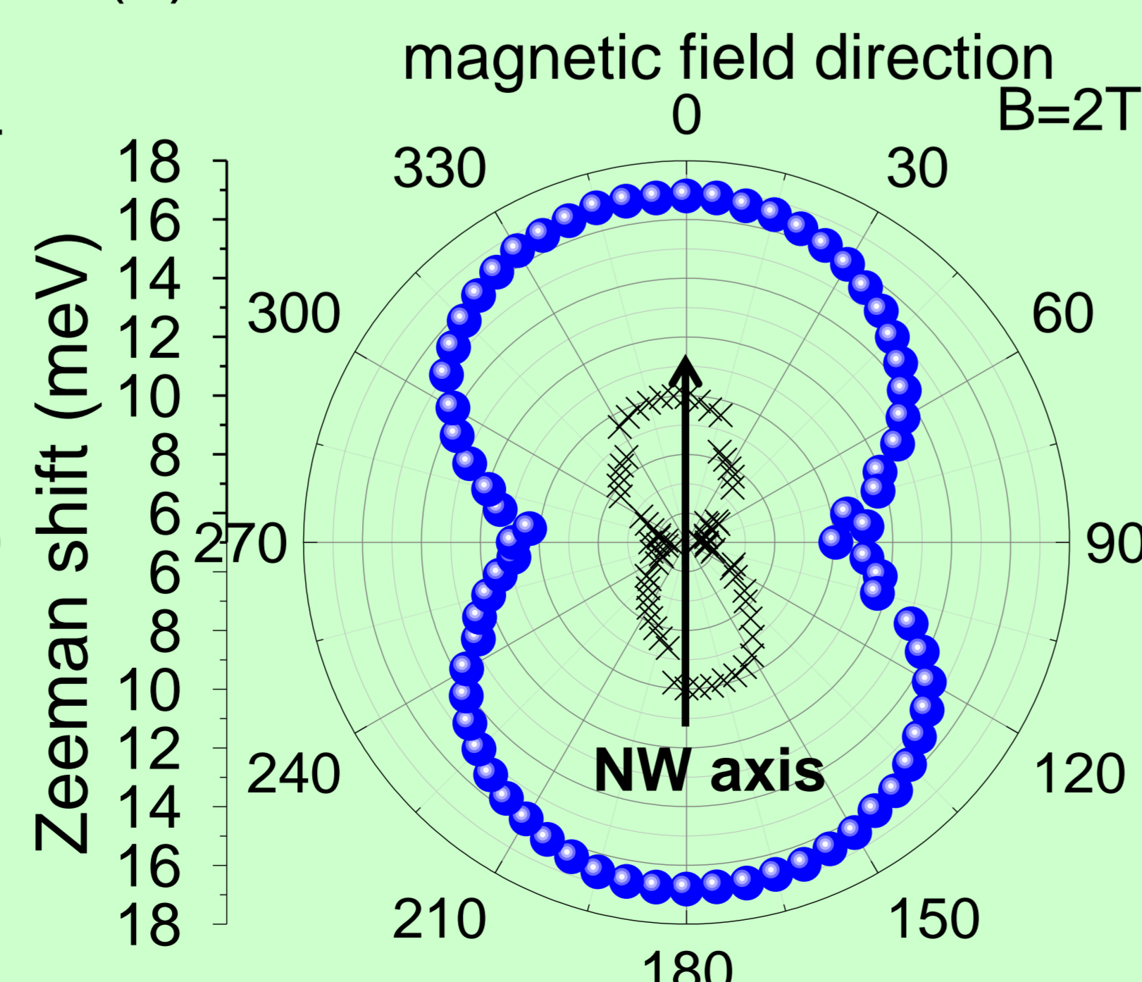
Fig. 5 Zeeman shift at |B| = 2T = \text{const} as a function of the field rotation angle for two individual (Cd,Mn)Te/(Cd,Mg)Te nanowires emitting at (a) 1.678 eV and (b) 1.728eV. Solid black arrows shows the NW axis determined from linear polarization anisotropy of the emission. T = 1.8K excitation with 515nm line and P=1μW
