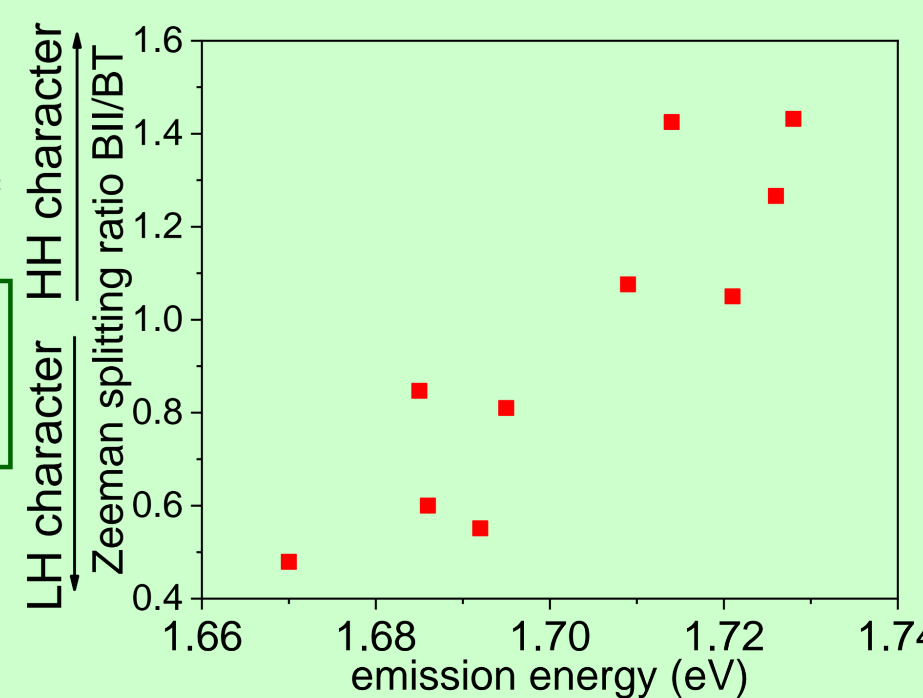
(b) line at 1.728 eV - HH-character
